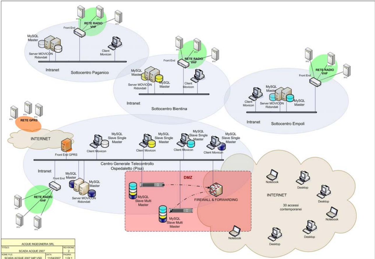
The Acque Spa remote control system architecture
