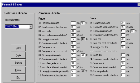
An example of the CIP system's wash parameter settings. Solutions are provided in the form of recipes to allow maximum management flexibility.
