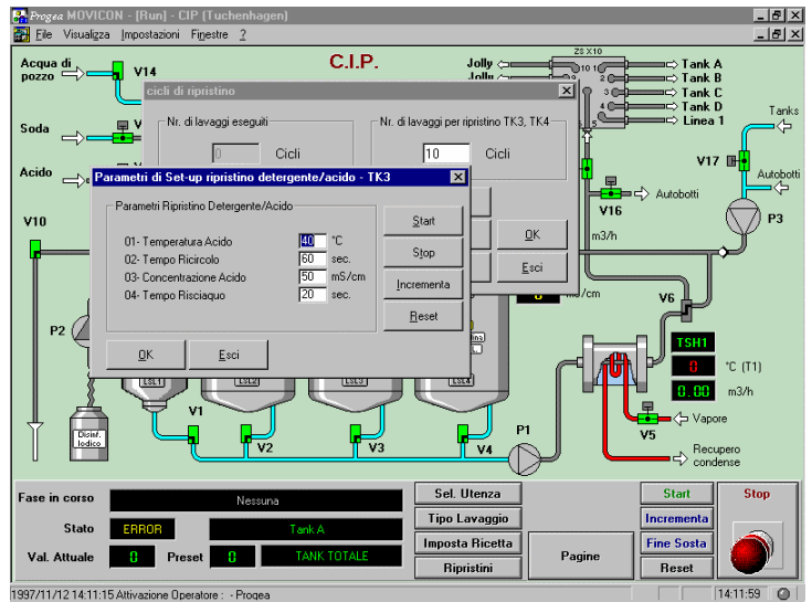
One of the Movicon application screens for supervising and controlling the dairy sanitization system
