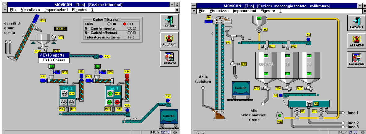
A Movicon dropdown window containing manual plant actuator commands
