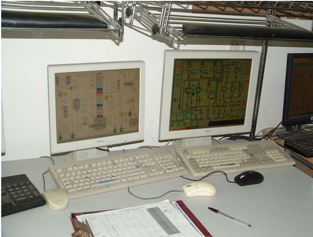
The Biodiesel plant Control Room. The plant workers can control the whole process using the redundant Movicon supervision workstations.
