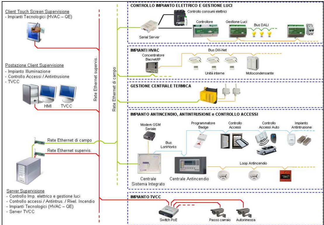
Figure 1 – Supervision system layout and connections
