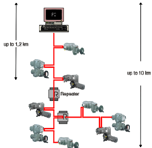
Photo B: A diagram of the Auma-Matic valves connected in a bus network, governed by the Movicon application
