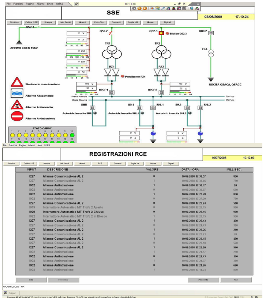
A screen showing events recorded in chronological order. The PLC records events in chronological order which are then displayed in their exact sequence in the supervisor.
